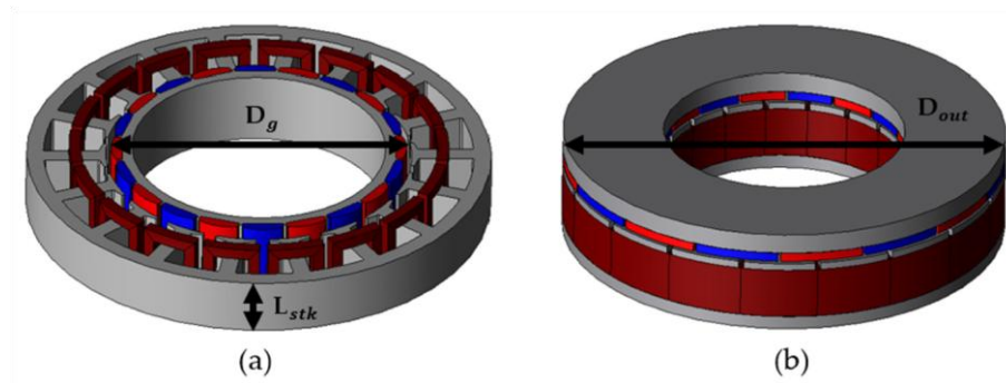
Figure 1. Motor types by magnetic path: (a) radial flux motor and (b) axial flux motor.
