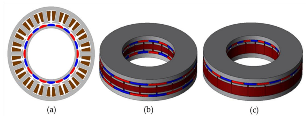
Figure 5. The 200-W-class motor for collaborative robot joints: (a) conventional radial flux motor; (b) single-rotor single-stator-type motor; and (c) double-rotor single-stator-type motor.
