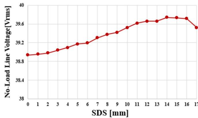
Figure 11. No-load line voltage of single-rotor single-stator type as SDS increases.
