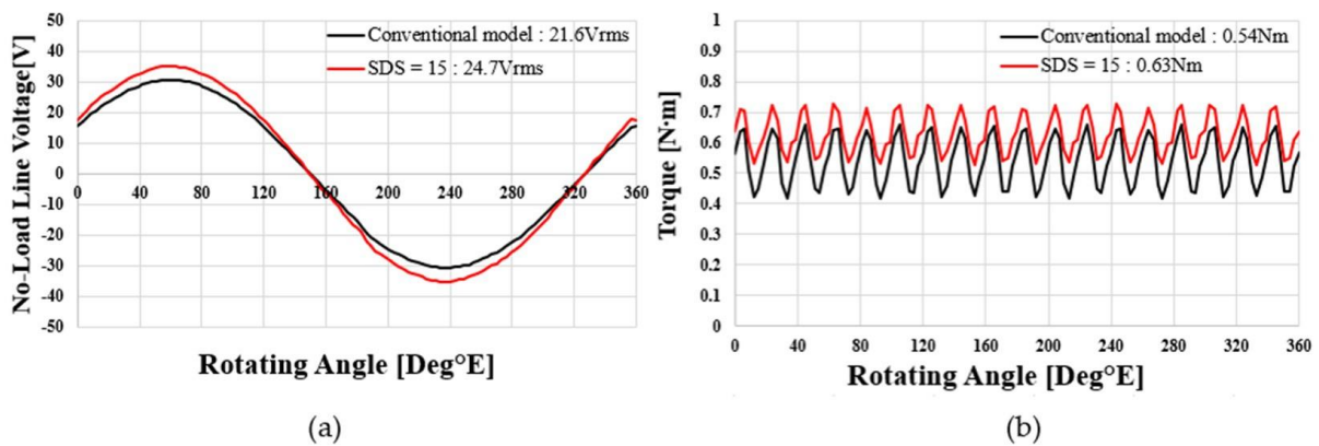
Figure 18. Shaft torque of double-rotor single-stator type under load according to SDS.
