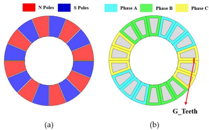
Figure 7. Existing shape: (a) magnet shape and (b) stator winding layout and spacing variable G\_Teeth .
