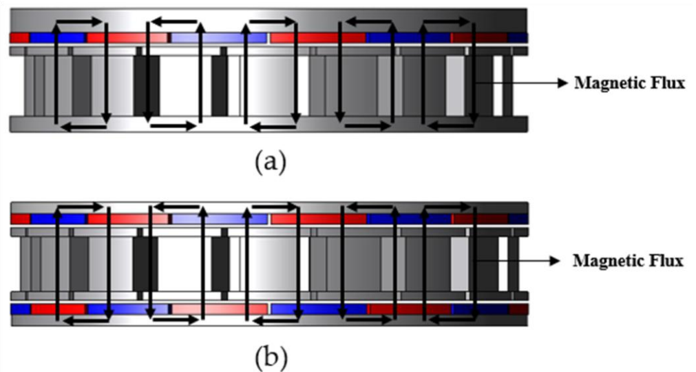
Figure 2. Magnetic path of axial flux motor: (a) single-rotor single-stator type and (b) double-rotor single-stator type.
