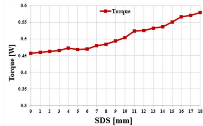
Figure 17. Load loss of double-rotor single-stator type according to SDS.
