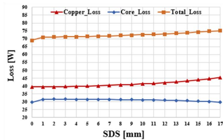
Figure 12. Load loss of single-rotor single-stator type according to SDS.
