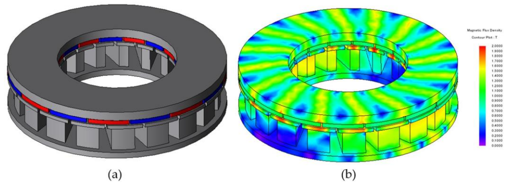
Figure 15. Final shape of single-rotor single-stator type (SDS = 11); (a) shape (b) magnetic flux density under load.
