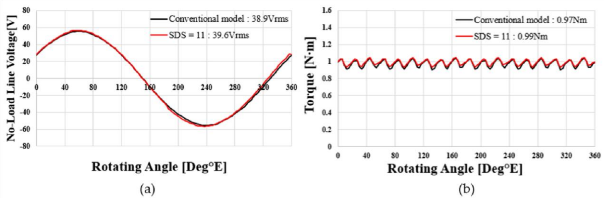
Figure 14. Performance comparison of single – rotor single – stator – type conventional model and SDS = 11 model: (a) no – load line voltage and (b) air gap torque waveform at load.
